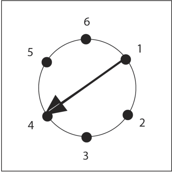
Figure 3: A simple digraph.
