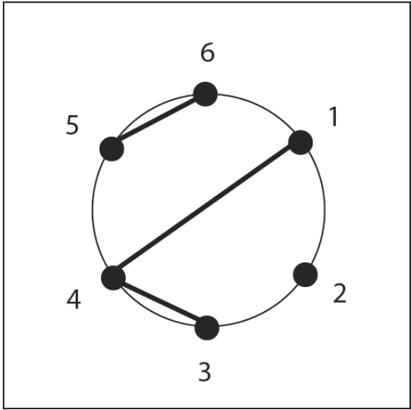
Figure 2: A simple graph.
